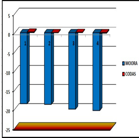
Figure 3: Ranking of the choices utilizing decision-making processes MOORA and CODAS at a variable level of -5%
