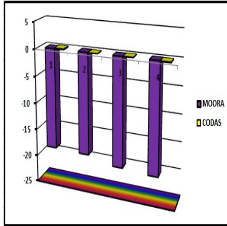
Figure 5: Ranking of the choices utilizing decision-making processes MOORA and CODAS at a variable level of -10%
