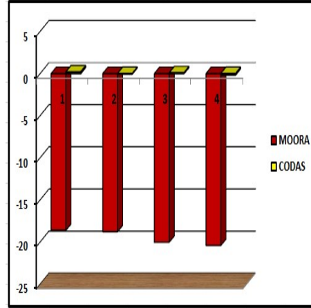
Figure 4: Ranking of the choices utilizing decision-making processes MOORA and CODAS at a variable level of +5%
