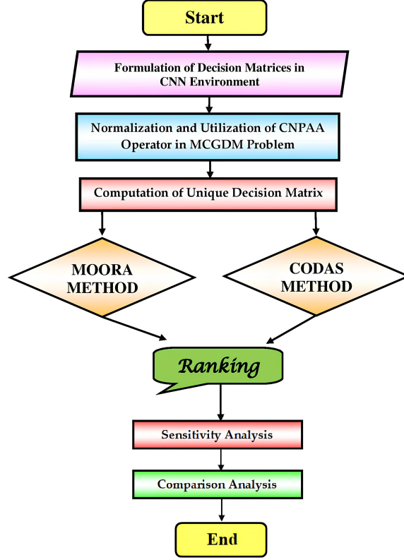
Figure 1: Method strategy of MCGDM problem for selecting an effective action for unlocking the potential of BEVs in West Bengal
