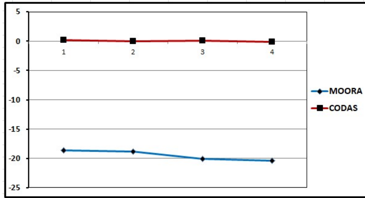
Figure 2: Ranking of the choices utilizing decision-making processes MOORA and CODAS
