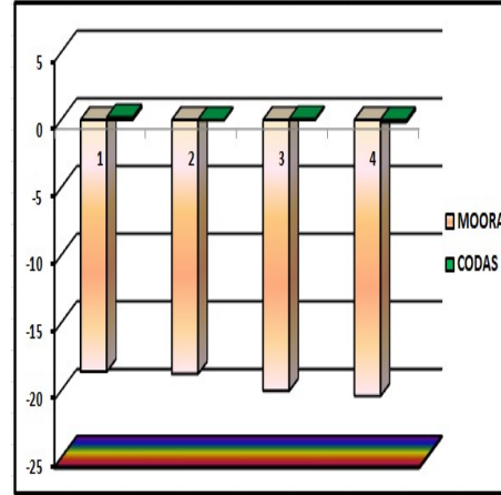
Figure 6: Ranking of the choices utilizing decision-making processes MOORA and CODAS at a variable level of +10%
