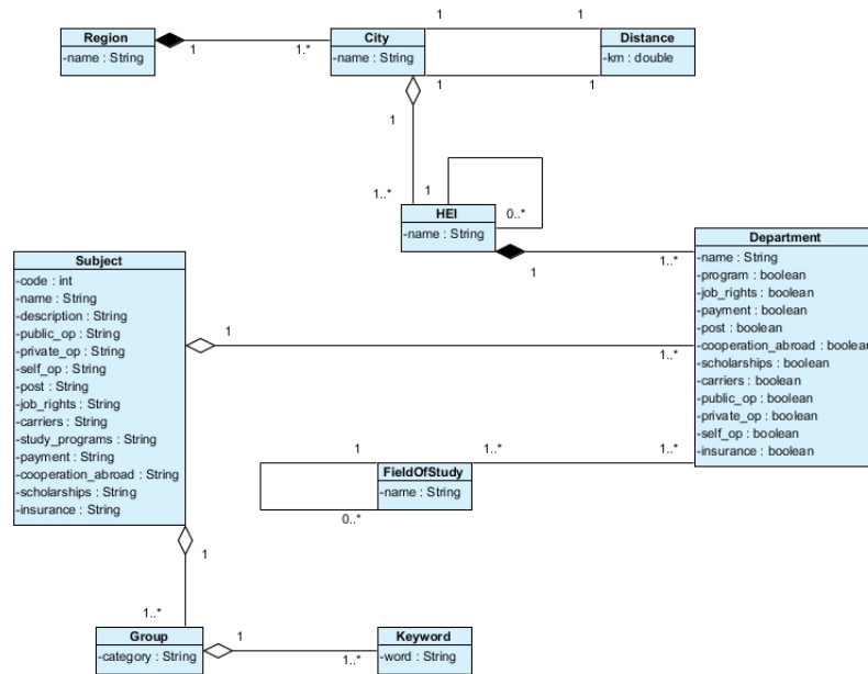
Figure 2: Class diagram
