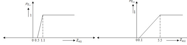
Figure 11: Lower-level membership functions defined as simple linear
