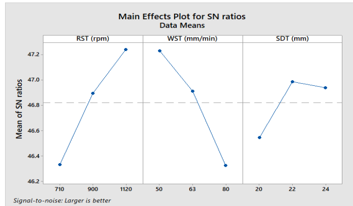
Figure 2: S/N ratio graphical plot- ultimate tensile strength
