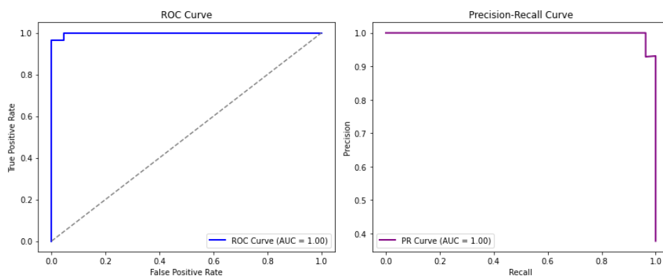
Figure 4: ROC and PR curves of the proposed model
