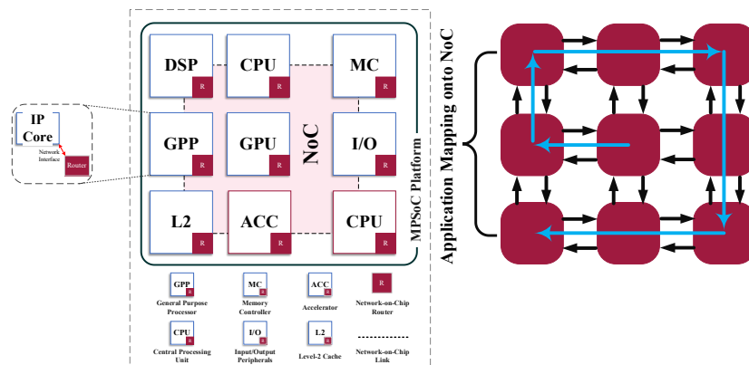
Figure 1: NoC-based MPSoC architecture with schematic diagram for mapping applications per IP Core
